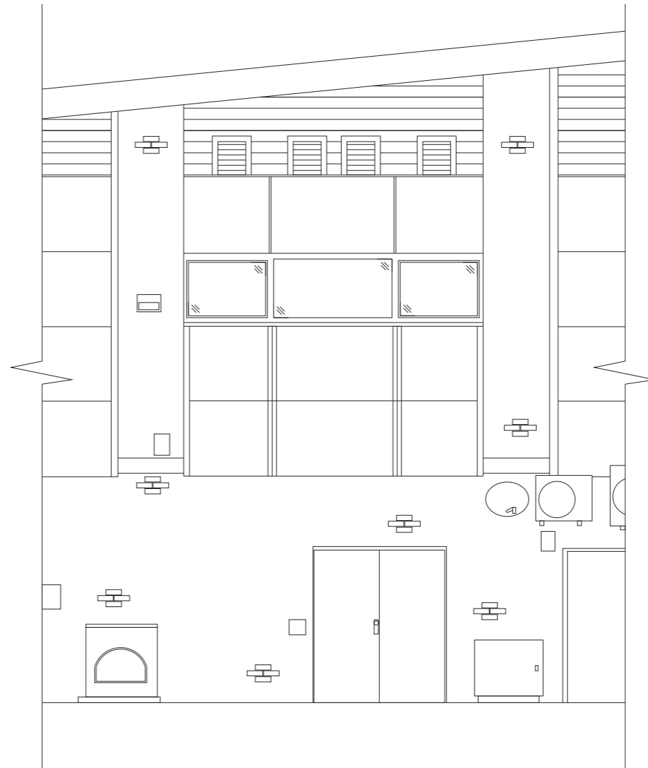
REAR ELEVATION
